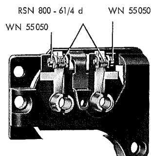
Fig. 13 Motorschild links
